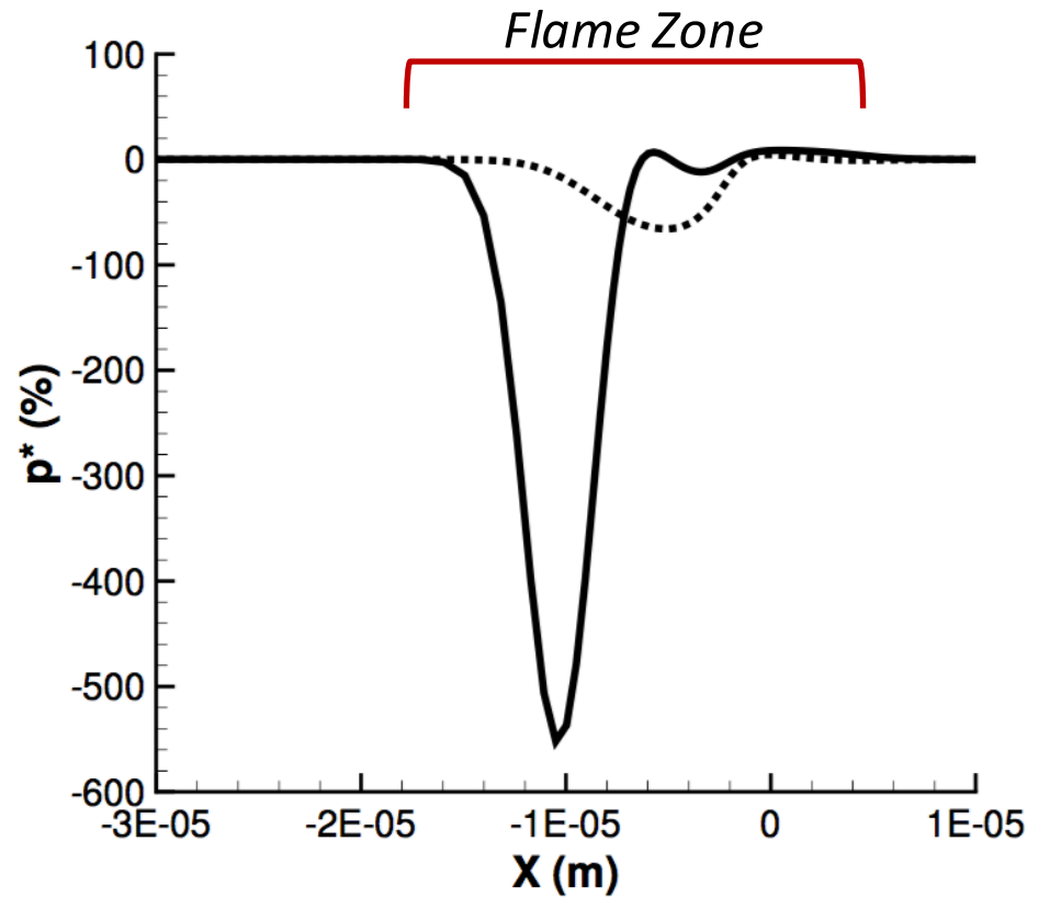
Non-Premixed Flame
