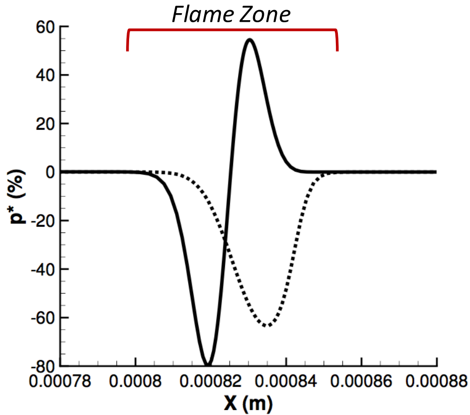
Premixed Flame
